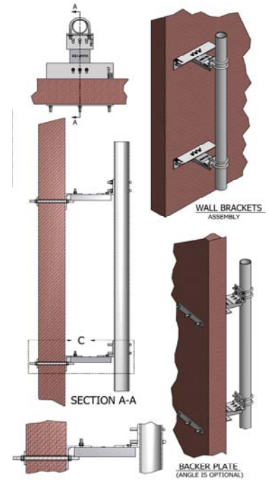
WPBGX512-73114 WITH 12" EXTENSION UNP
